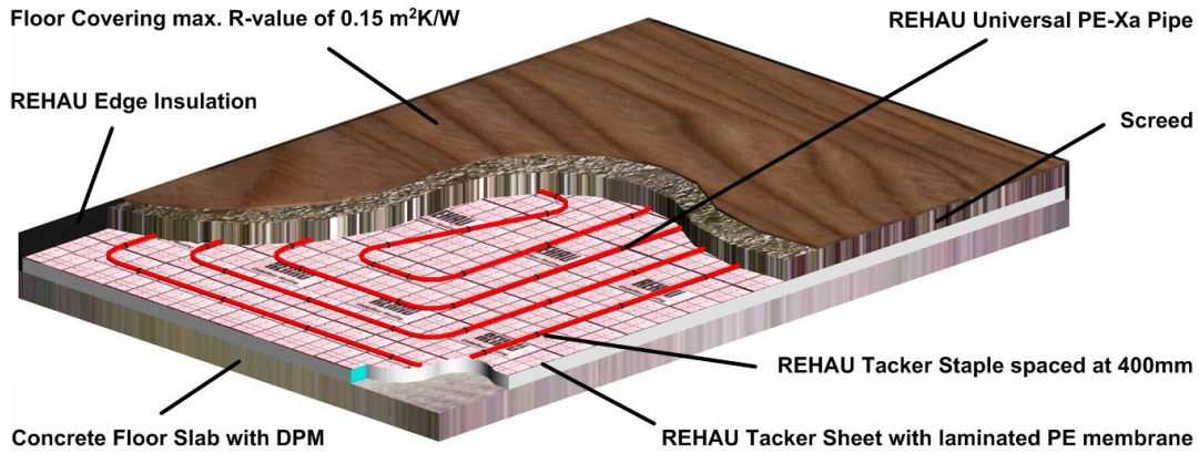
Typical Floor Structure for REHAU Tacker Sheet System
