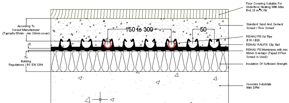
Typical Floor Structure for REHAU RAUfix System
