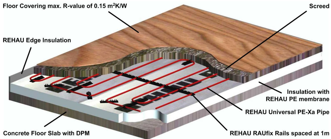
Typical Floor Structure for REHAU RAUfix System
